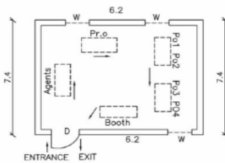
CAD Drawing.
