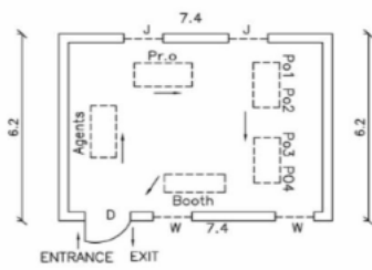
CAD Drawing.
