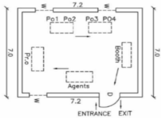
CAD Drawing.
