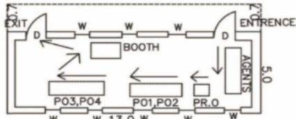
(3) CAD DRAWING
