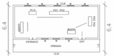
(3) CAD Drawing
