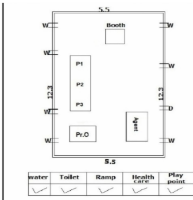
Cad View
