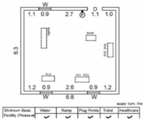
CAD DRAWING
