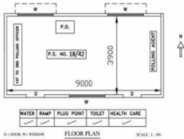
FLOOR PLAN
