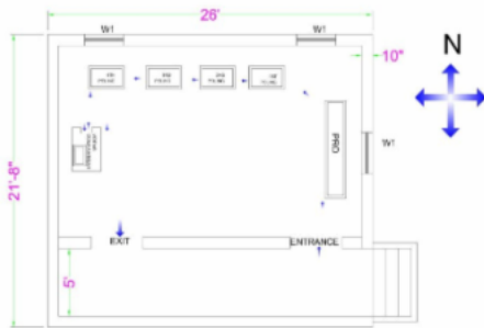
Cad View
