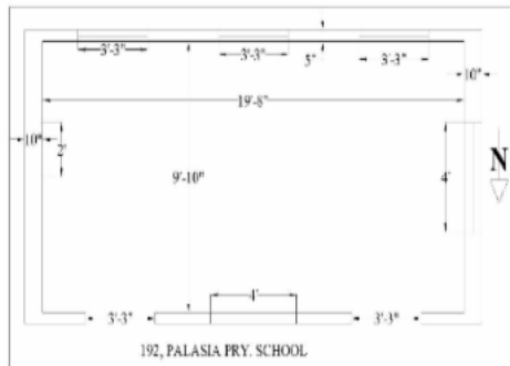
Cad View
