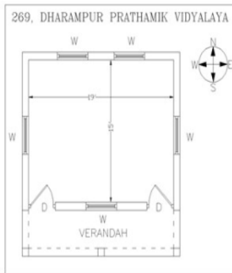
Cad View
