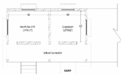
Plan of Chamni F.P.School (Part No.279) (Not To Scale)
