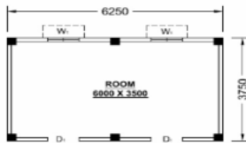
GROUND FLOOR PLAN SCALE = 1 : 100
