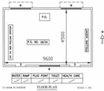
FLOOR PLAN
