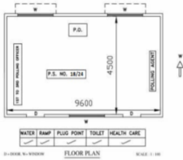
FLOOR PLAN
