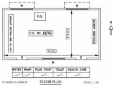
FLOOR PLAN
