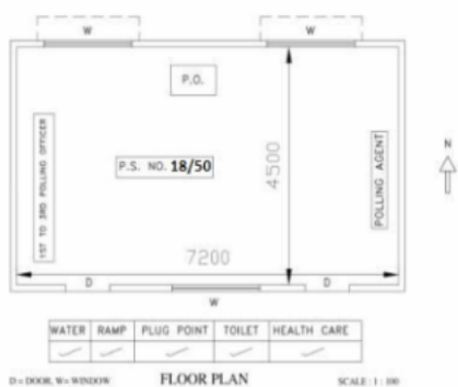
FLOOR PLAN
