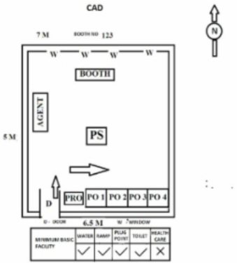
Cad View
