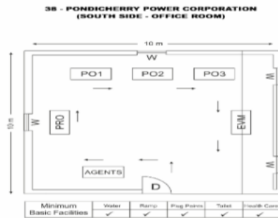
Cad View
